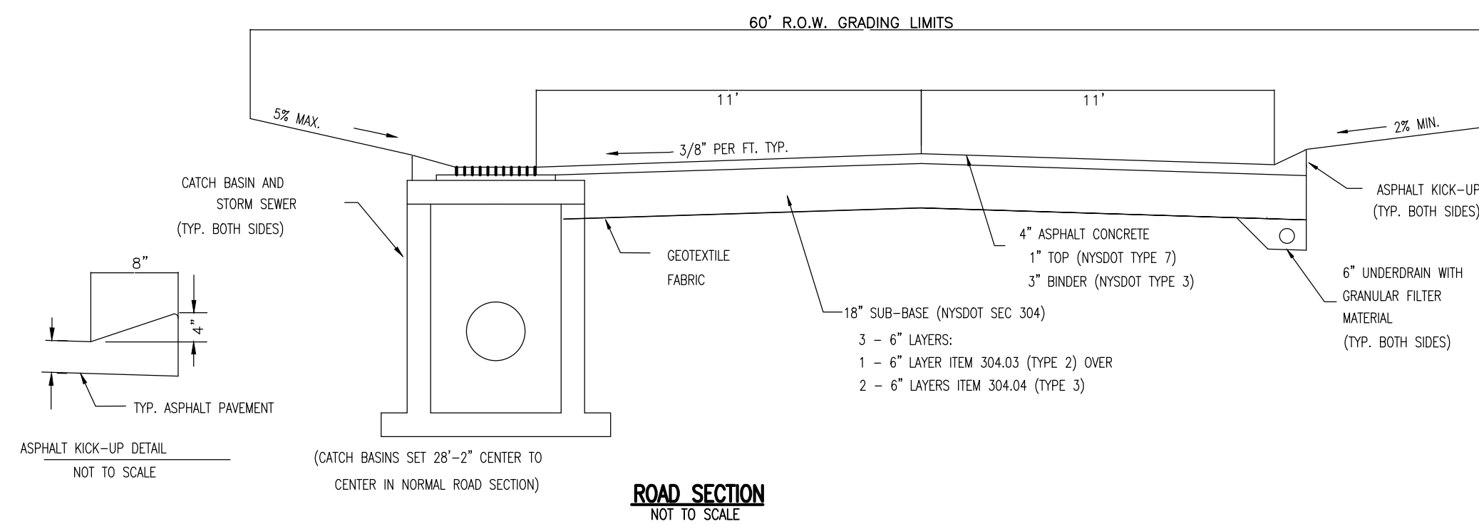
ROAD SECTION (NOT TO SCALE)
