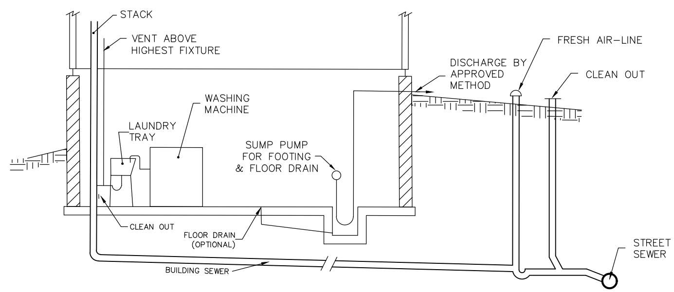
TYPICAL PLUMBING LAYOUT FOR WET SEWER CONNECTION (NOT TO SCALE)
