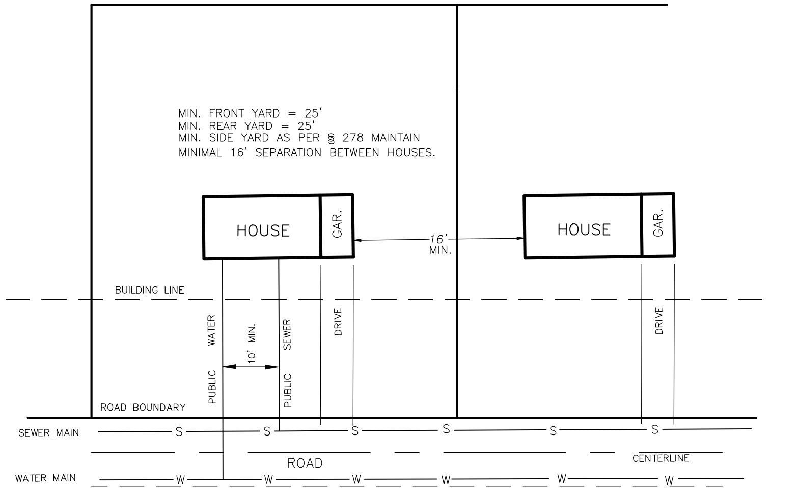
TYPICAL LOT LAYOUT (NOT TO SCALE)
